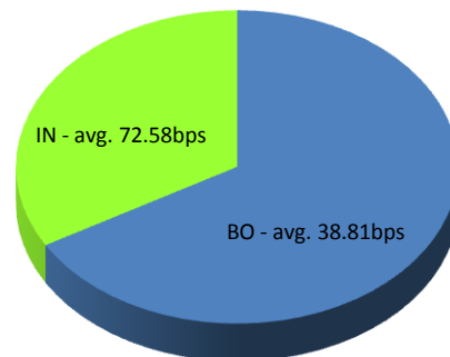
SUNFRONT(8934.T)
