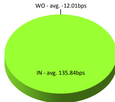
SUNFRONT(8934.T)
