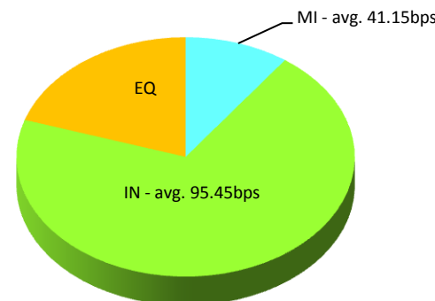
KOSAIDO(7868.T)
